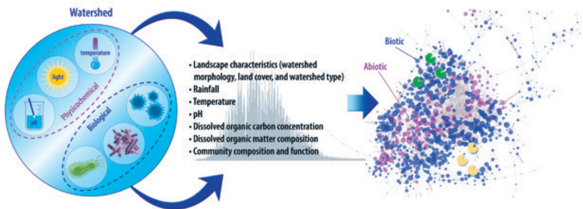
Fig. 1. Identifying “marker” transformations and reactions will require studying the coupling between the hydroclimatic, biological, and landscape conditions that influence dissolved organic matter degradation. [Tfaily Lab, University of Arizona]
