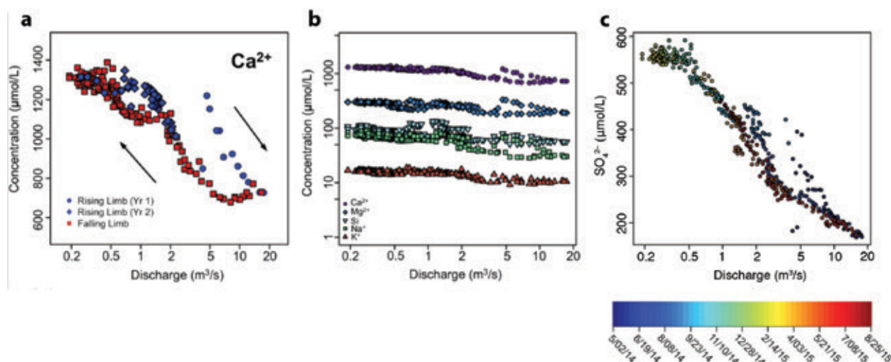
Fig. 3.12. Examples of Concentration-Discharge (C-Q) Relationships at the East River Pumpphouse Site in Colorado. (a) Semi-log calcium ions ( \text{Ca}^{2+} ) show an annual hysteresis pattern, (b) log-log C-Q for all base cations indicating chemostatic behavior, and (c) sulfate ( \text{SO}_4^{2-} ) C-Q. Blue points represent the rising limb of the hydrograph, red points represent the falling limb, and first-year and second-year rising limbs are denoted by shape. [Adapted from Winnick, M. J., et al. 2017. "Snowmelt Controls on Concentration-Discharge Relationships and the Balance of Oxidative and Acid-Base Weathering Fluxes in an Alpine Catchment, East River, Colorado," Water Resources Research 53 (3), 2507–23.]
